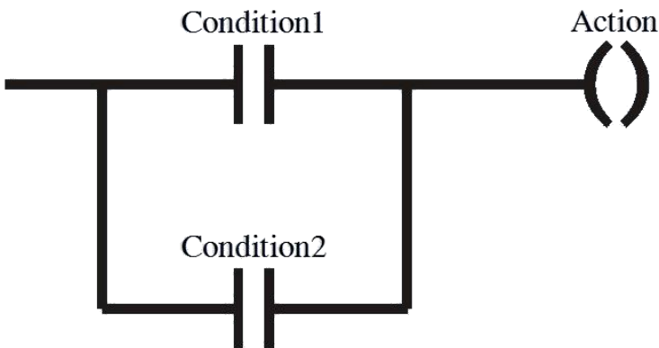
Fig.7 – OR Logic Diagram
