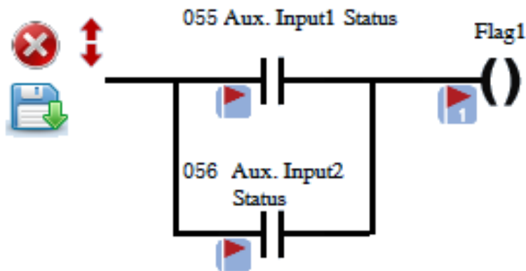
Fig.8 – OR Logic Example Diagram
