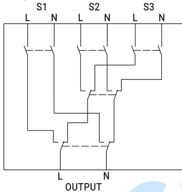
Fig.5 – Internal Transfer Diagram
