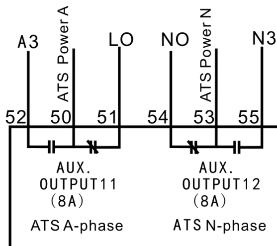
Fig.4 – Wring of ATS Supplied by Any of S1, S2, S3
