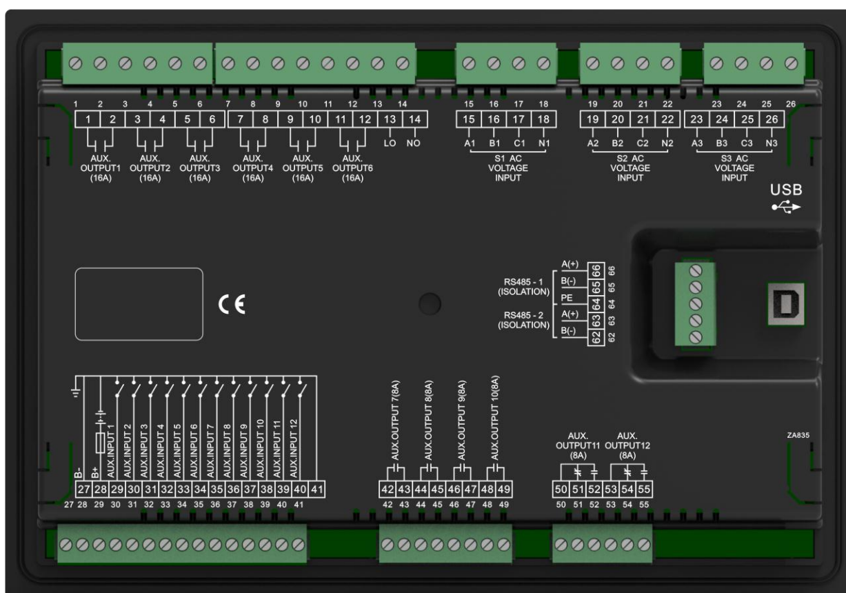
Fig.13 – Controller Rear Panel Drawing
