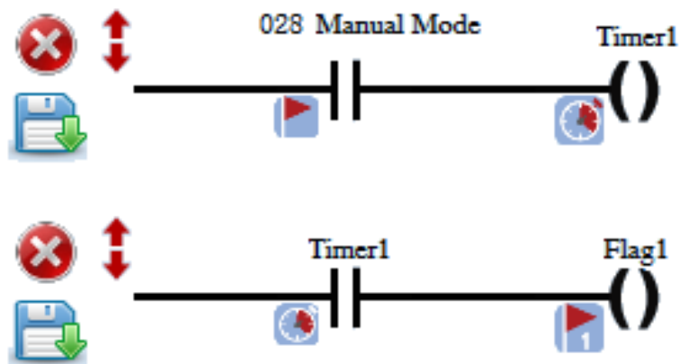
Fig.11 – PLC Example2 Logic
