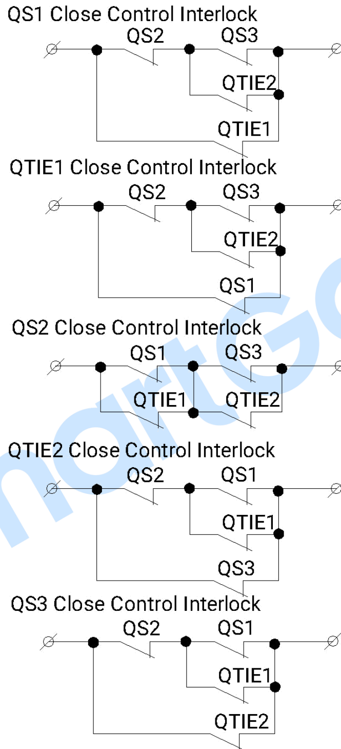
Fig.18 – 3P2B Electrical Interlock Logic Diagram
