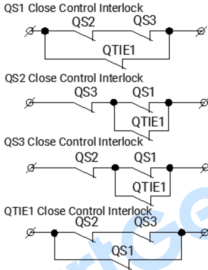
Fig.19 – 3P1B Electrical Interlock Logic Diagram
