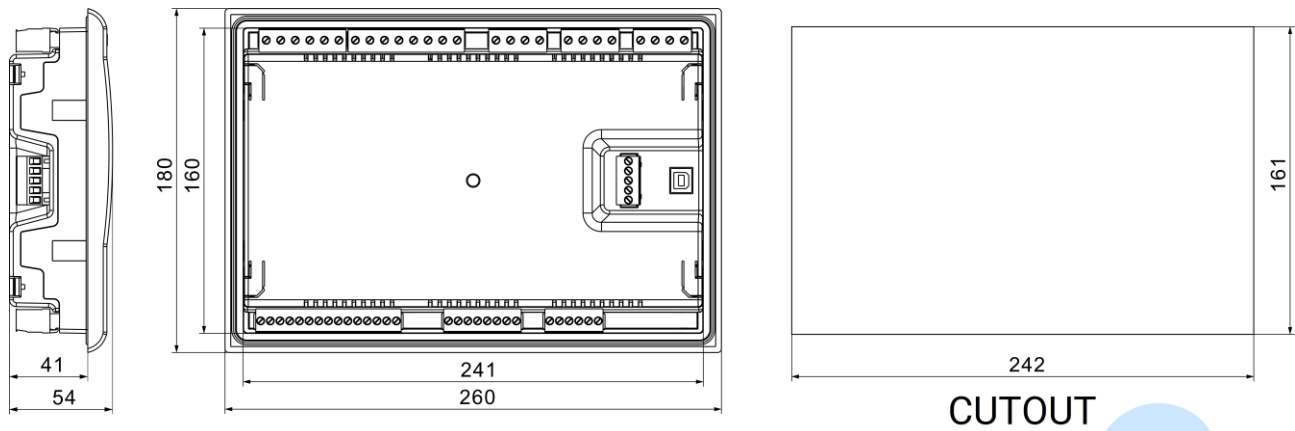
Fig.20 – Overall & Cutout Dimensions
