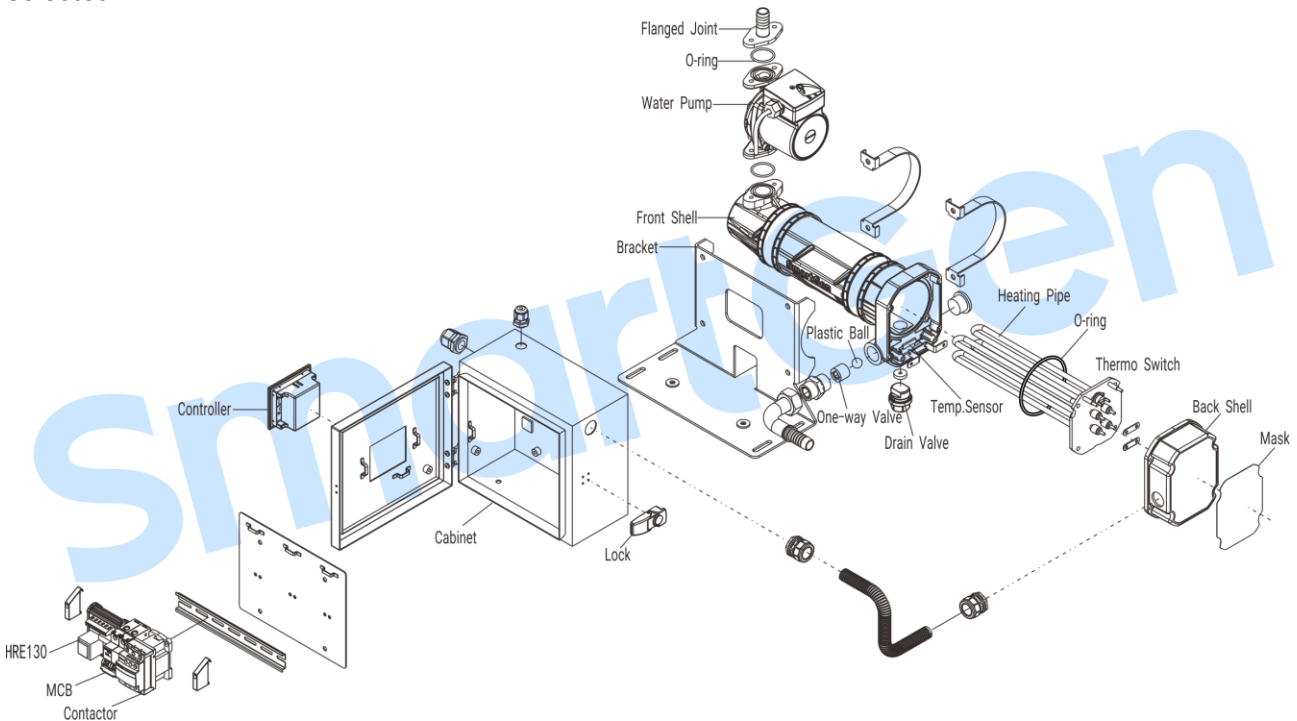
Fig. 4 – Assembly Structure
