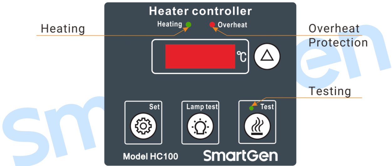
Fig.5– Operation Panel Drawing
