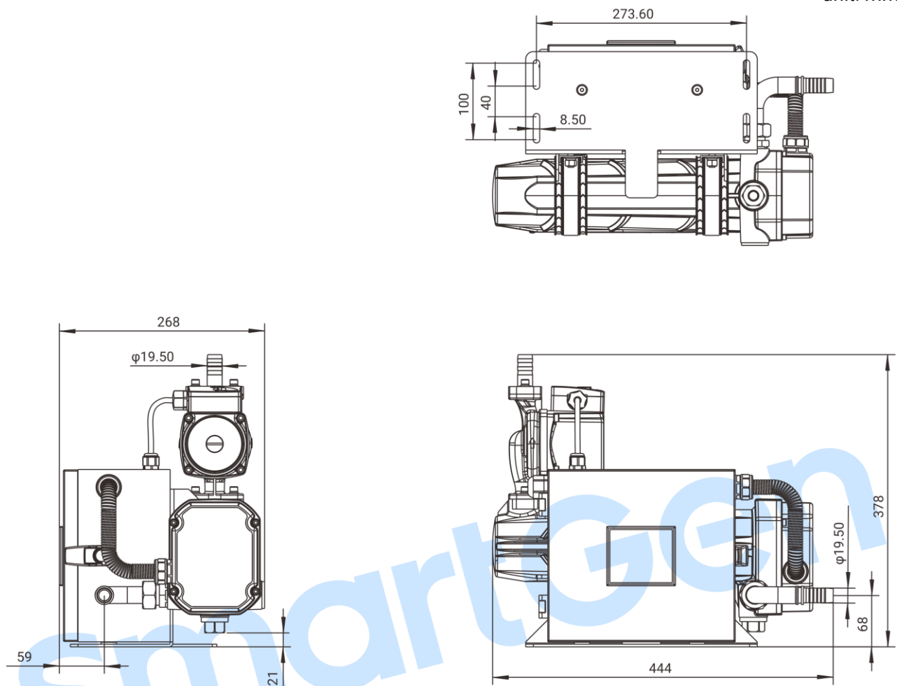
Fig.10 – Overall Dimensions
