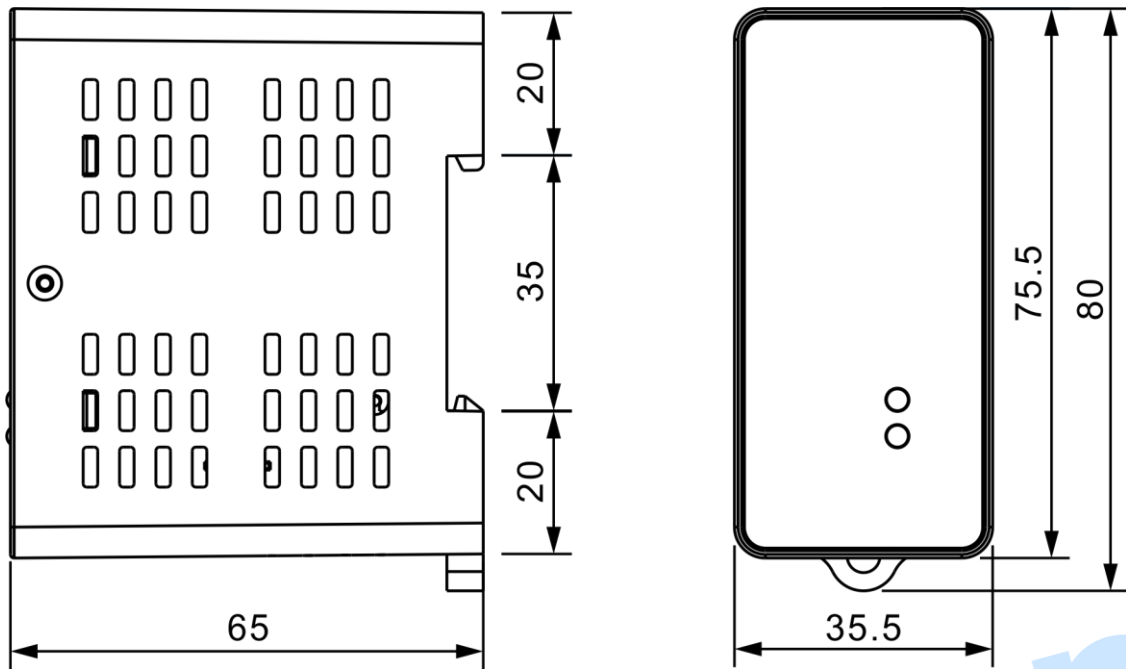
Figure 3 BAC1203VL Guide Rail Installation Size
