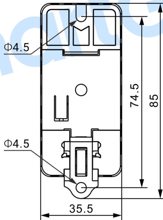
Figure 4 BAC1203VL Screw Installation Size
