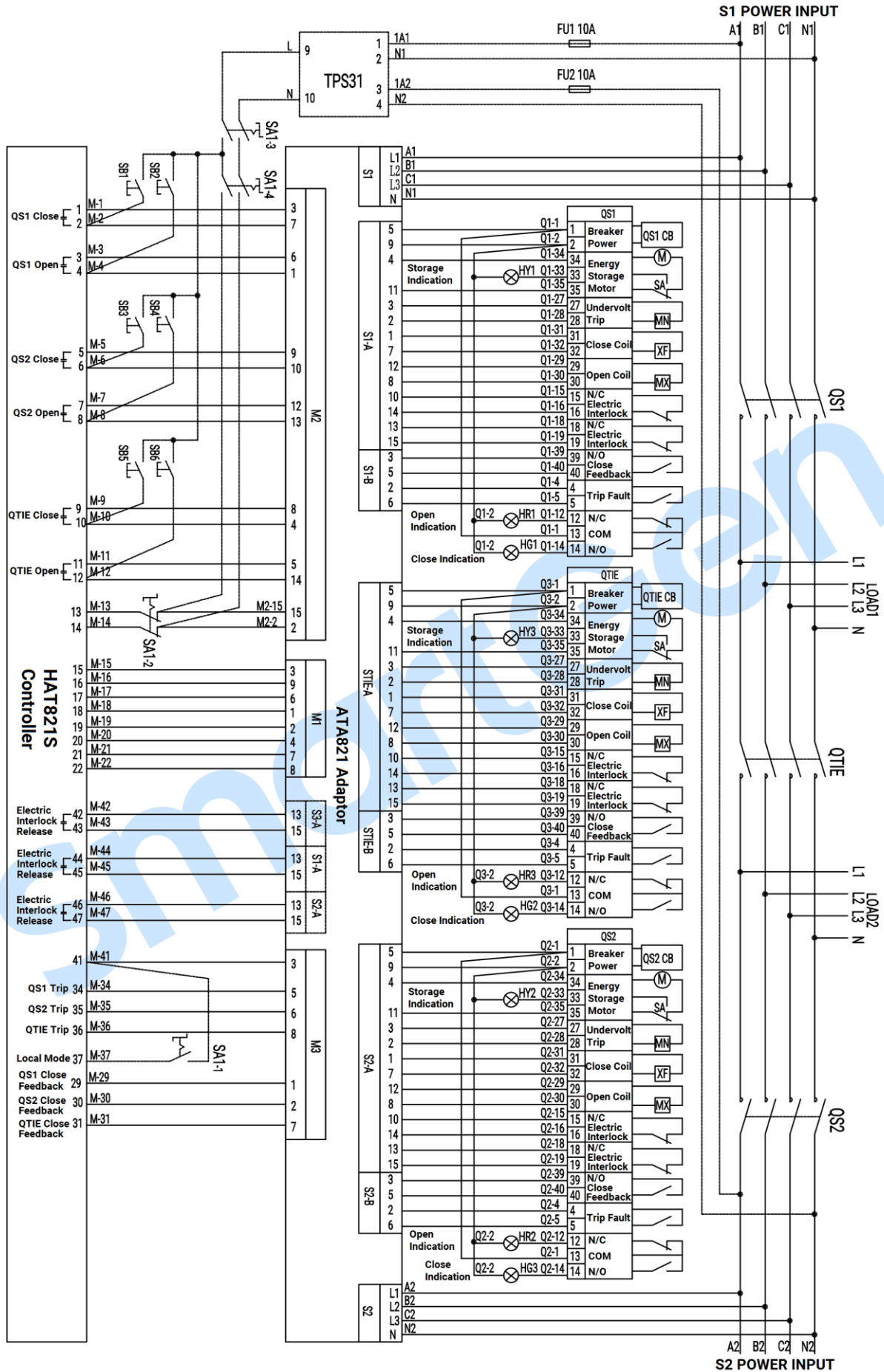
Fig.7 – Electric Interlock Release Application Diagram
