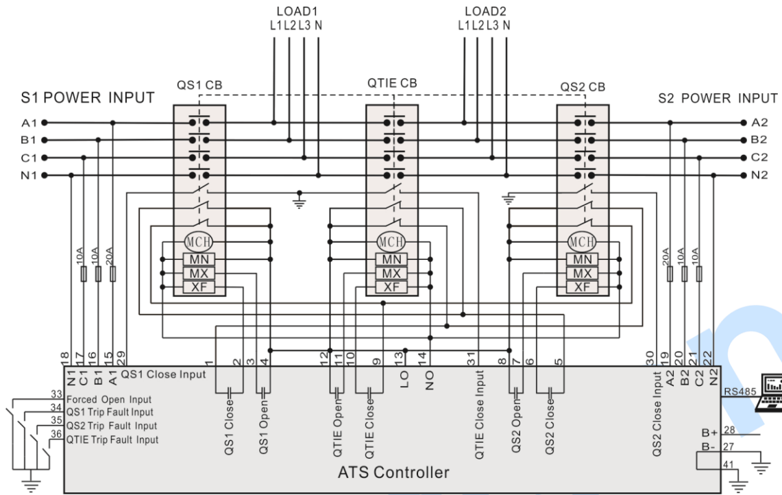
Fig.5 – Breaker Application Diagram 1 (Recommended)
