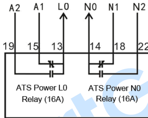
Fig.3 – Internal Wiring of ATS Power LO-NO Output
