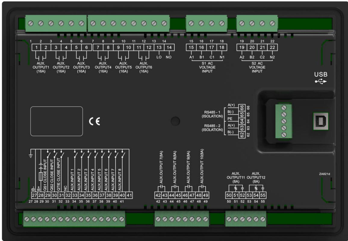
Fig.4 – Controller Rear Panel Drawing
