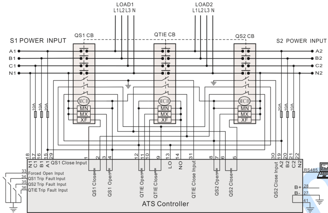
Fig.6 – Breaker Application Diagram 2
