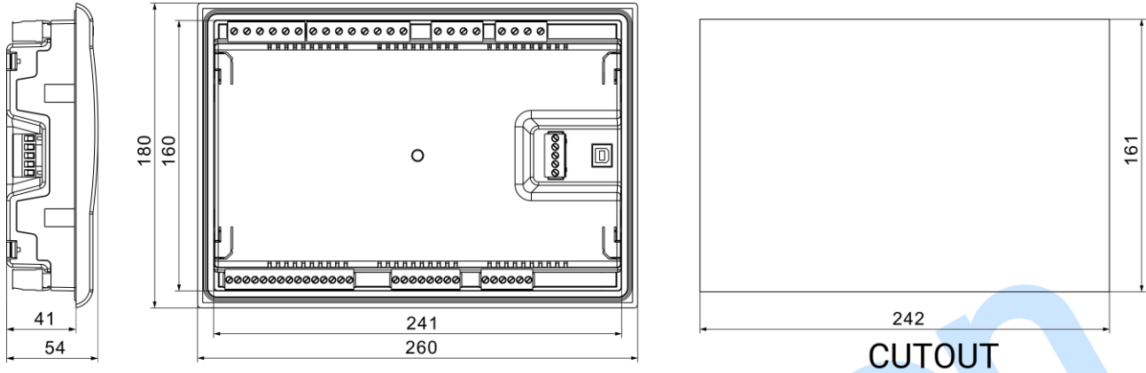
Fig. 8 – Overall & Cutout Dimensions
