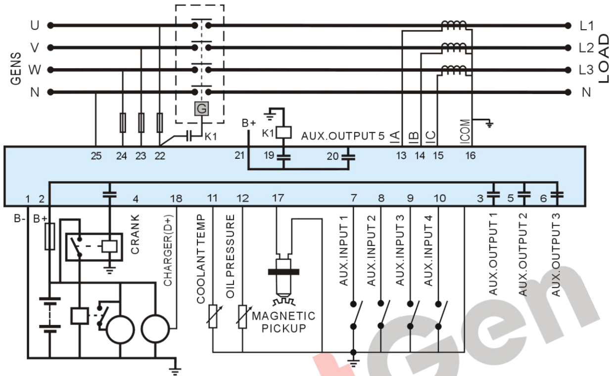
Fig. 4 HGM410N Typical Wiring Diagram
