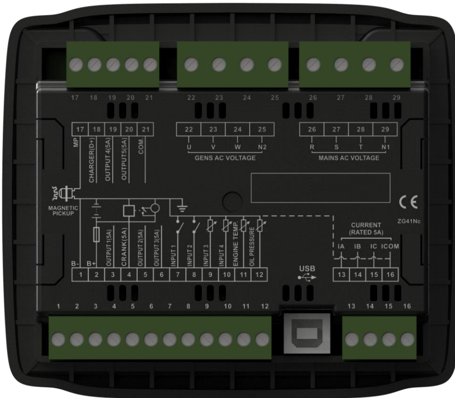
Fig. 3 Back Panel
