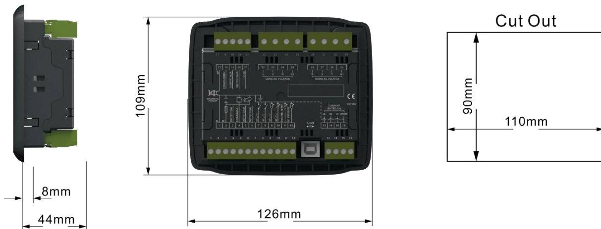
Fig. 8 Case Dimension and Cutout Size
