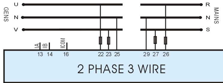
Fig. 7 2 Phase 3 Wire (HGM420N)
