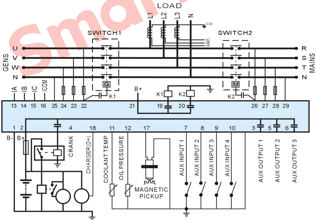
Fig. 5 HGM420N Typical Wiring Diagram
