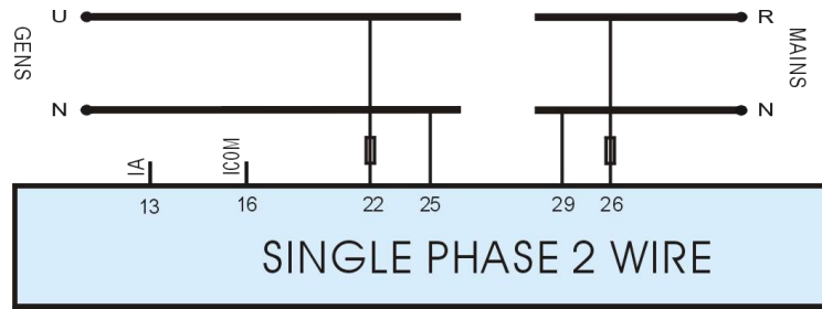
Fig. 6 Single Phase 2 Wire (HGM420N)
