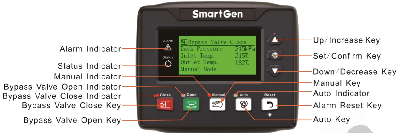
Fig. 1 - HEM4100EX Panel Indication
