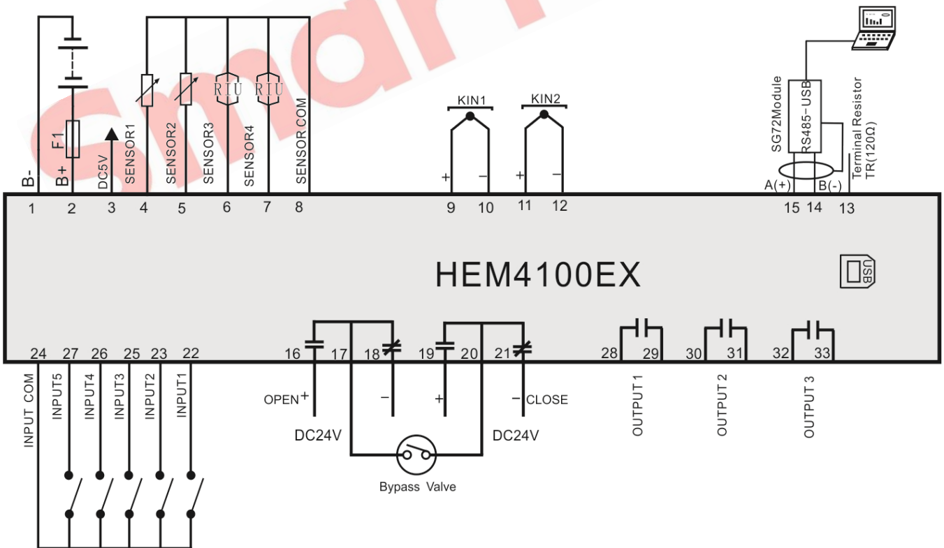
Fig. 8 - HEM4100EX Typical Application Diagram
