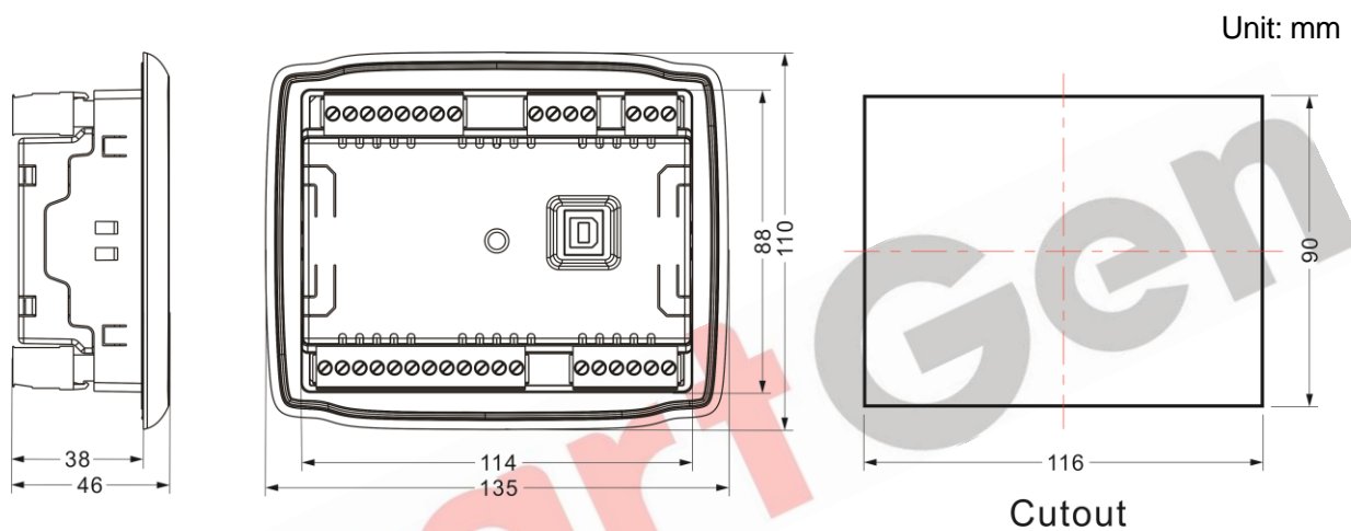
Fig. 9 - Case Dimensions and Panel Cutout
