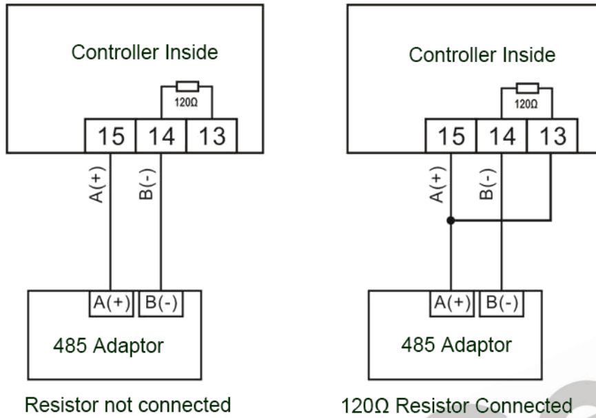
Fig. 7 - RS485 Connection Diagram
