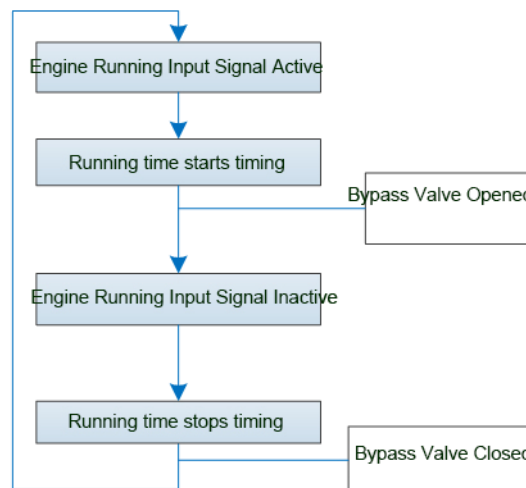
Fig. 3 - Engine Running Status Control Valve Open/Close Diagram
