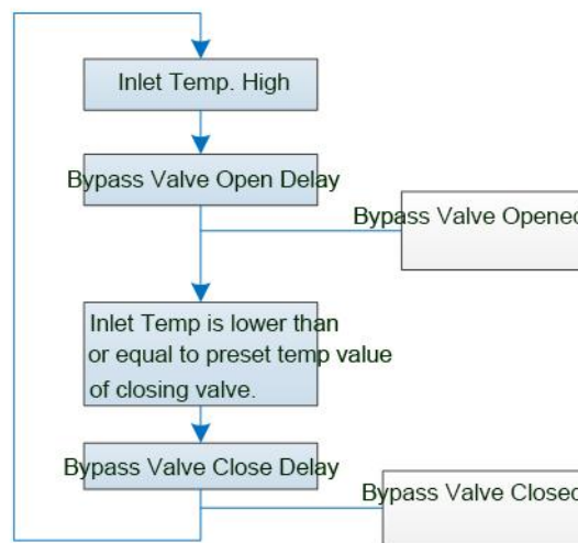
Fig. 2 - Inlet Temp Control Valve Open/Close Diagram
