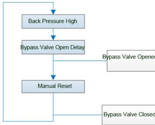
Fig. 4 - Back Pressure Control Valve Open Diagram
