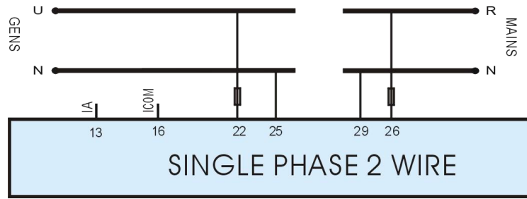
Fig. 7 Single Phase 2 Wire (HGM420N)
