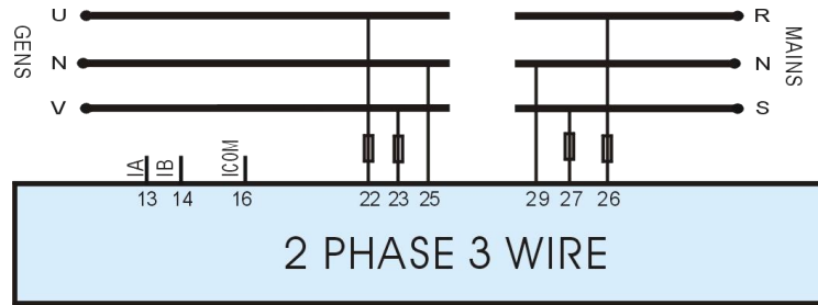
Fig. 8 2 Phase 3 Wire (HGM420N)
