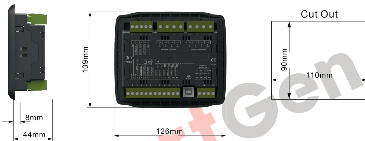
Fig. 9 Case Dimension and Cutout Size
