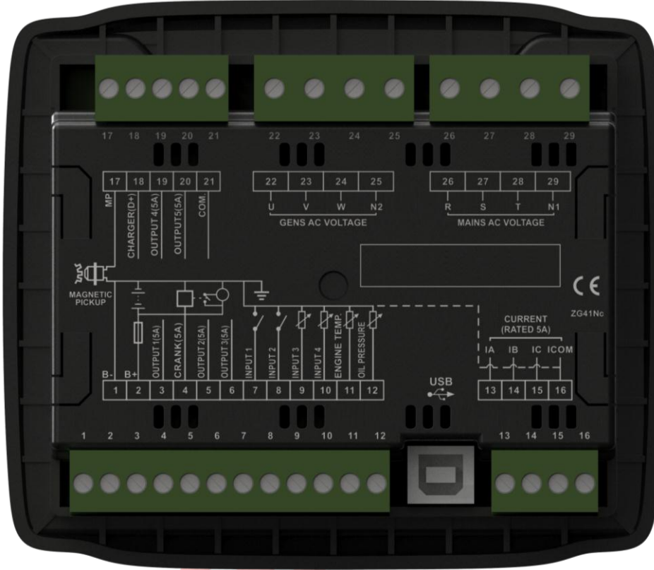
Fig. 3 Controller Back Panel
