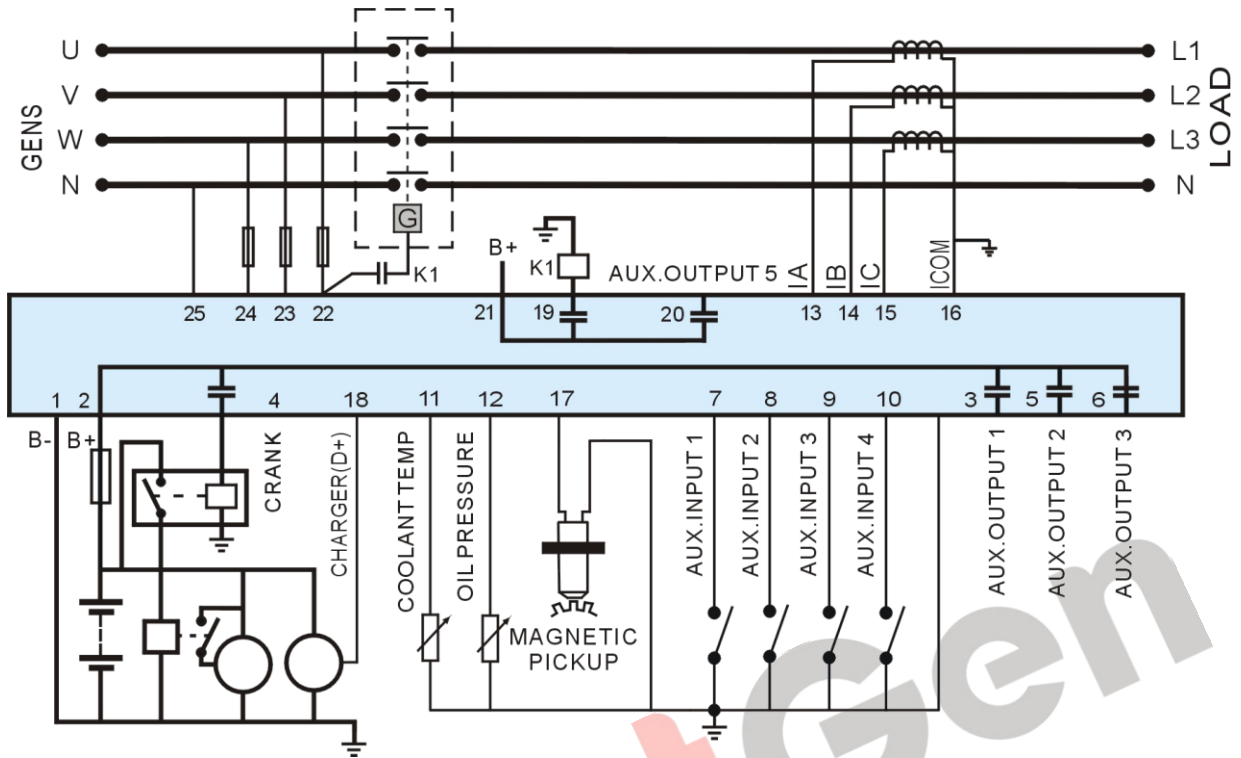
Fig. 5 HGM410N Typical Application Diagram
