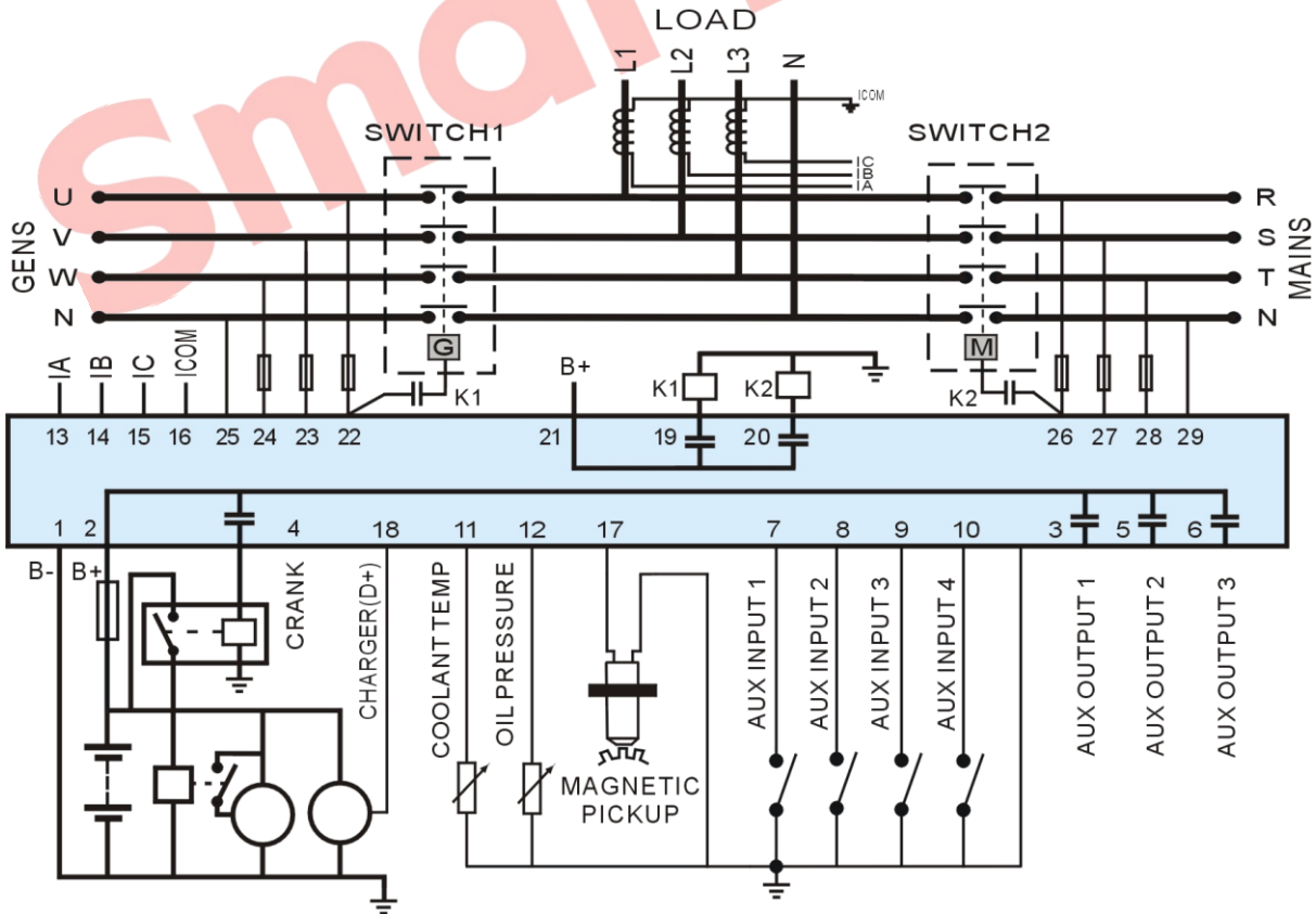
Fig. 6 HGM420N Typical Application Diagram
