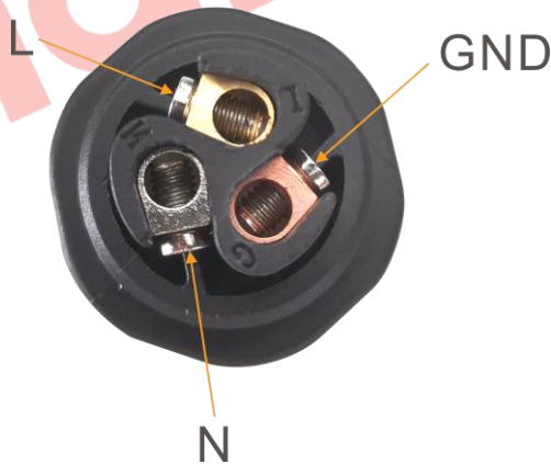
Fig. 5 Wire Connection
