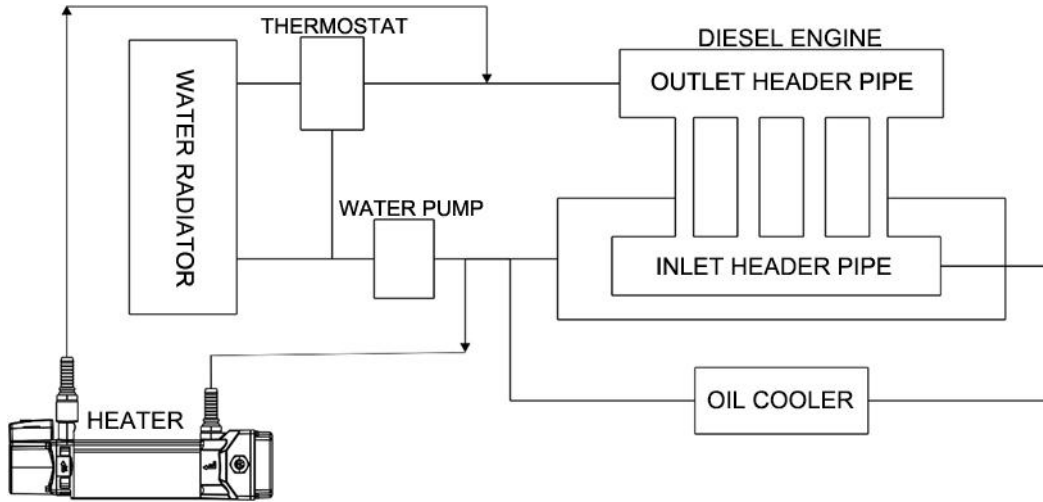
Fig. 1 - Installation Logic Diagram
